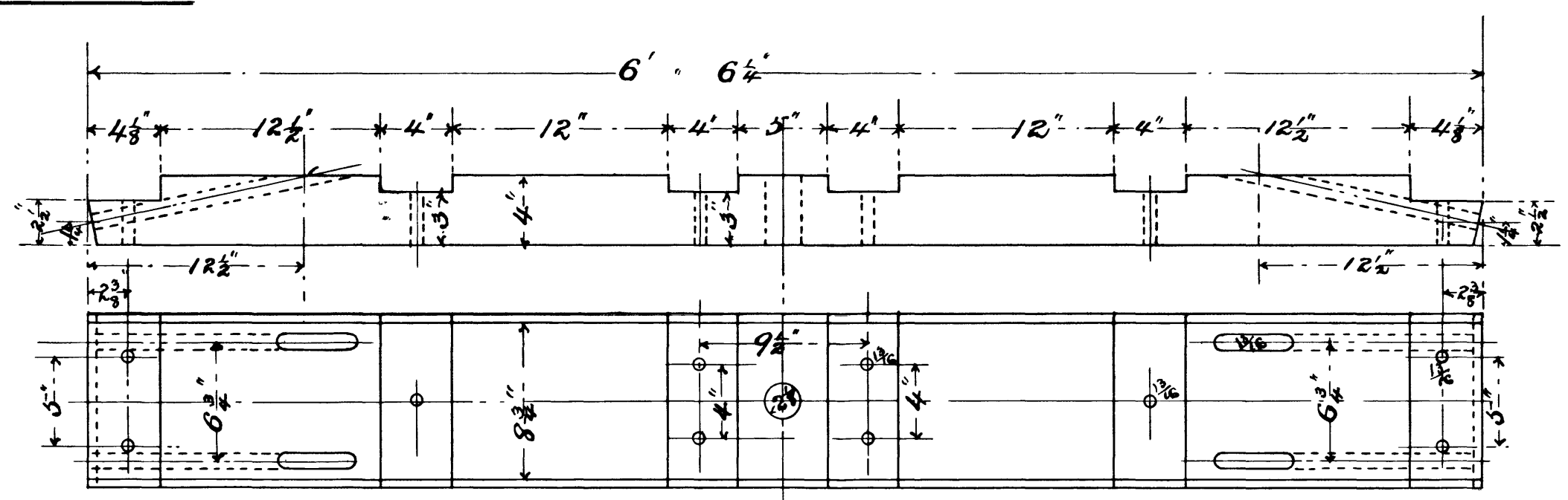
BODY BOLSTER
