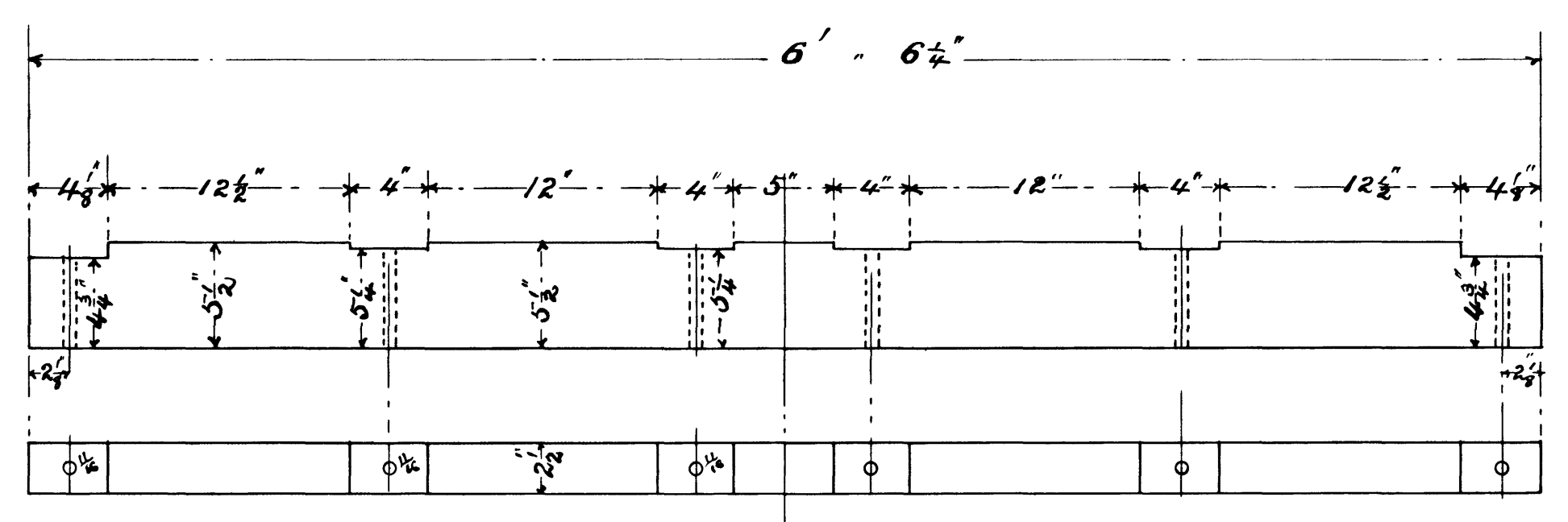
NEEDLE BEAM
