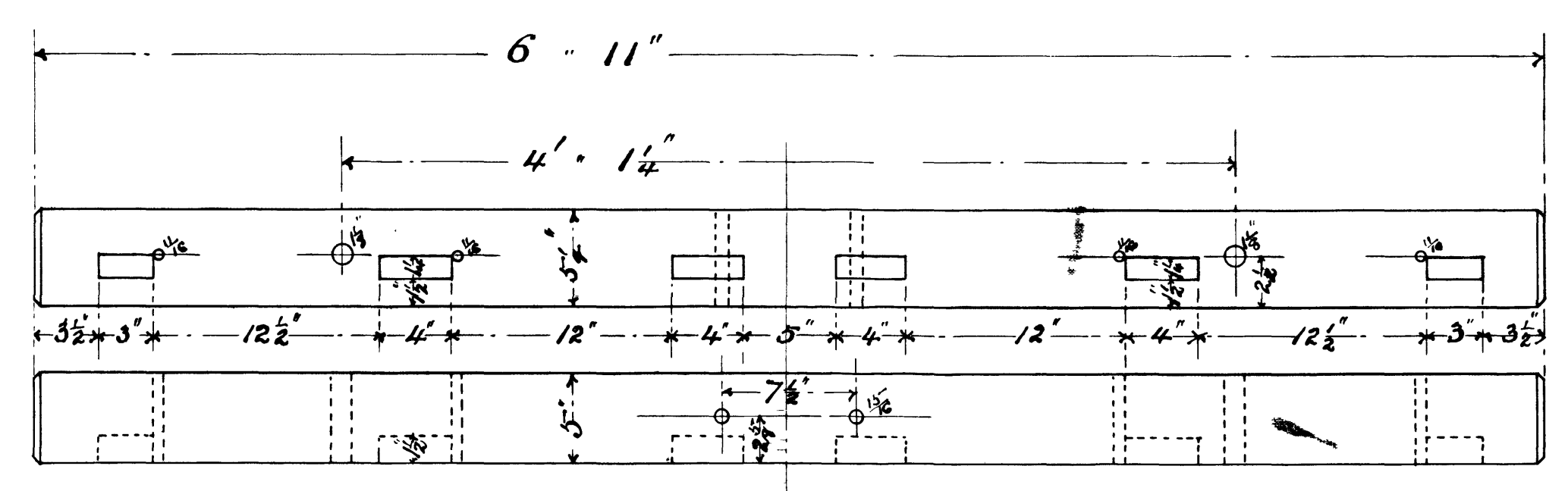
END SILL
