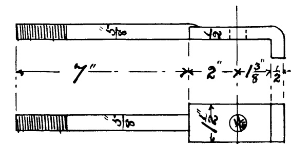
JOINT BOLT
