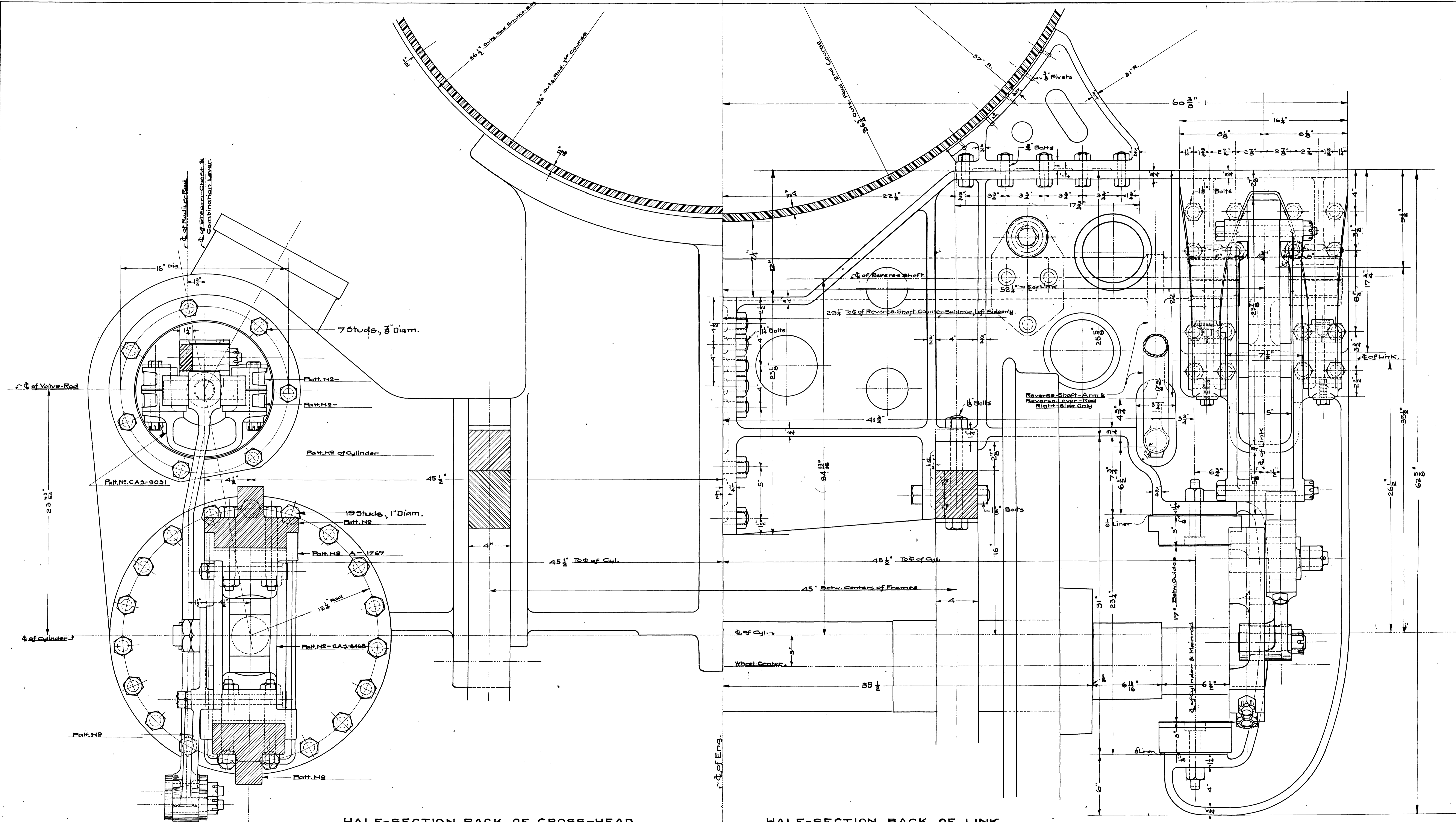
HALF-SECTION BACK OF CROSS-HEAD LEFT SIDE
