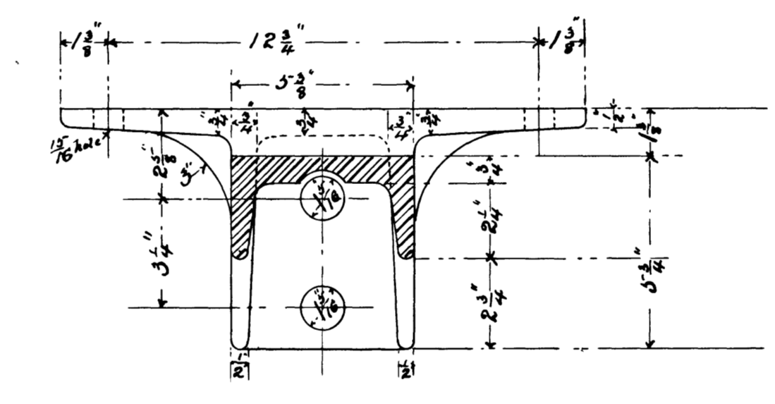
Section through A.A. Malleable Iron. Part of 6808.
