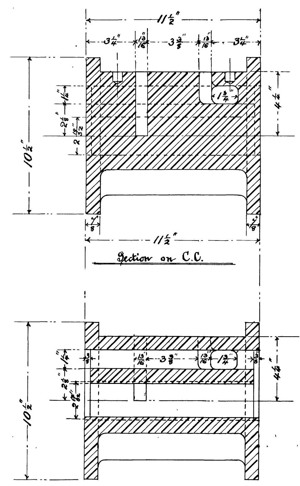
Section on C.C.
