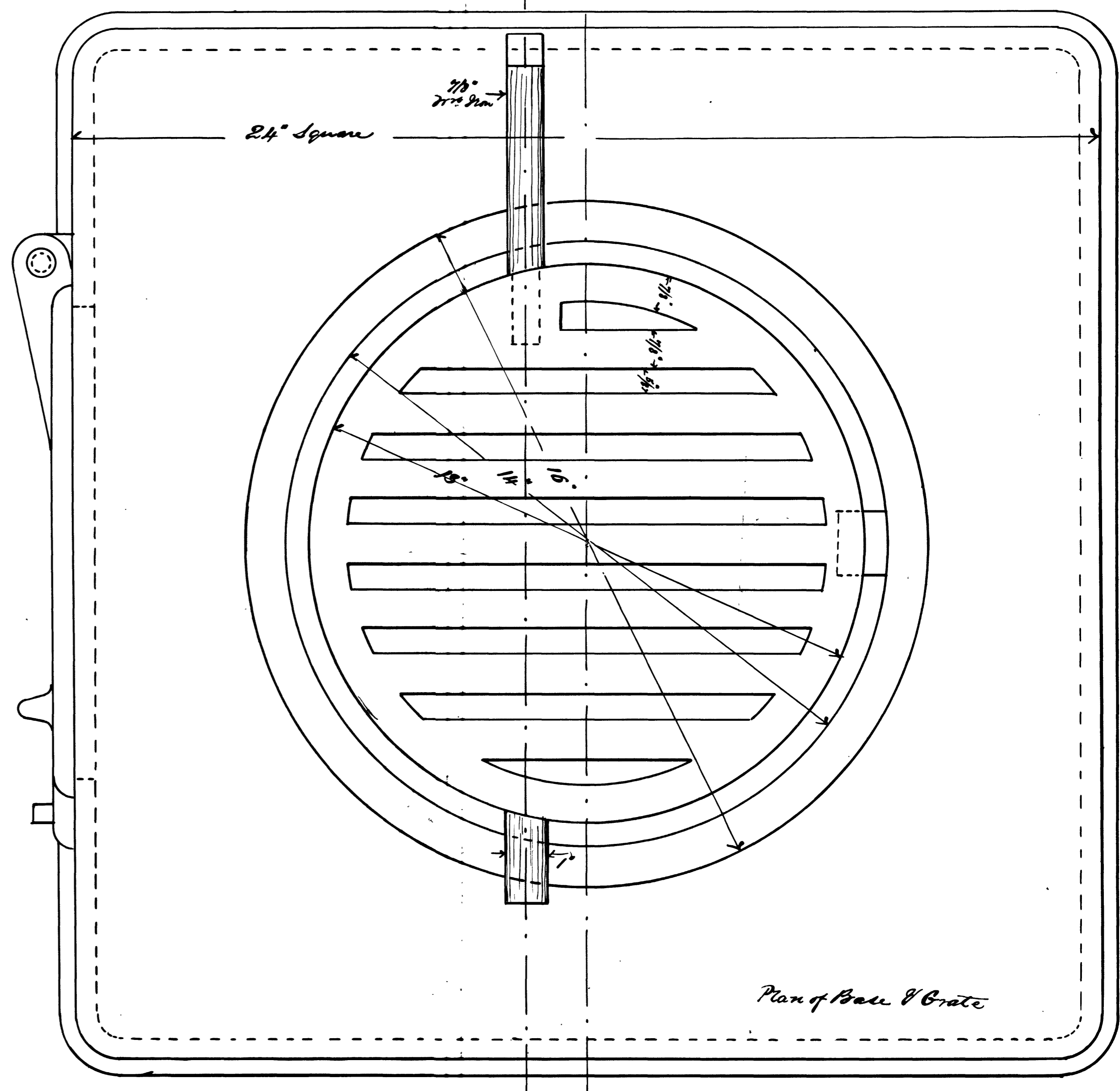
ORVY. Co Round House Coal Stove Scale Half Size
