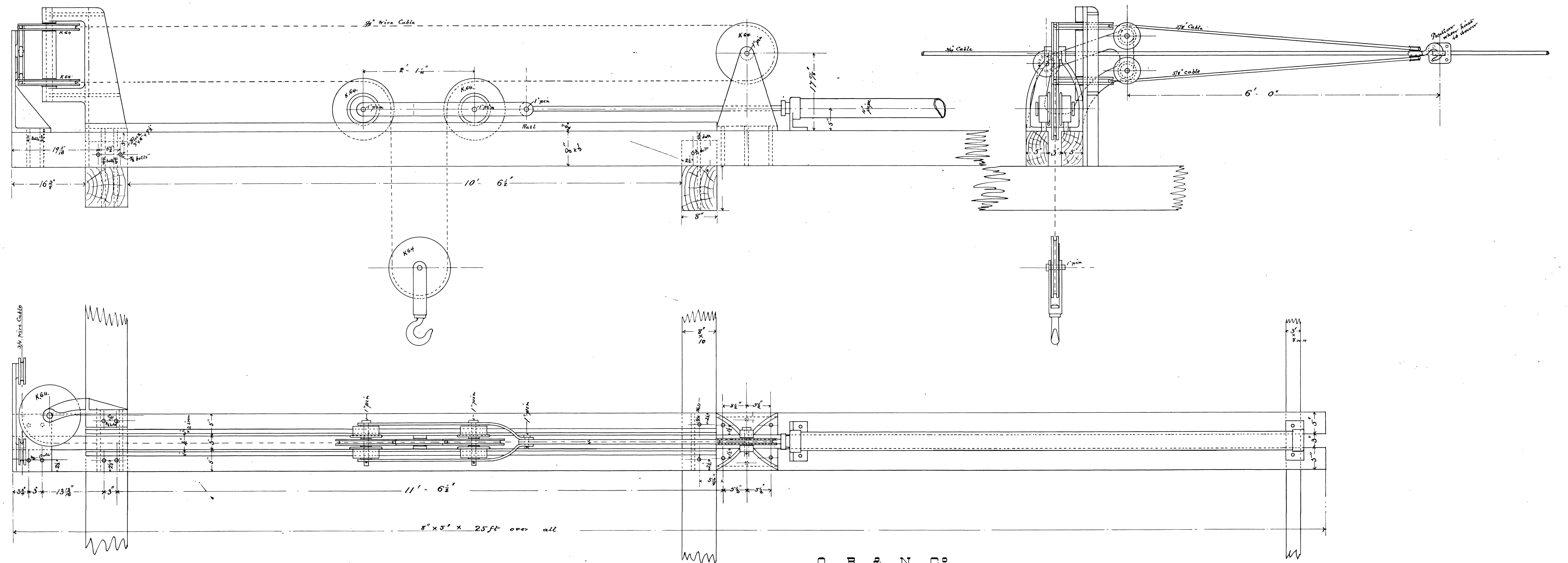
O R & N CO GENERAL ARRANGEMENT OF CAB HOIST Scale 1/2" = 1ft Astoria, Oregon, Dec 1896.
