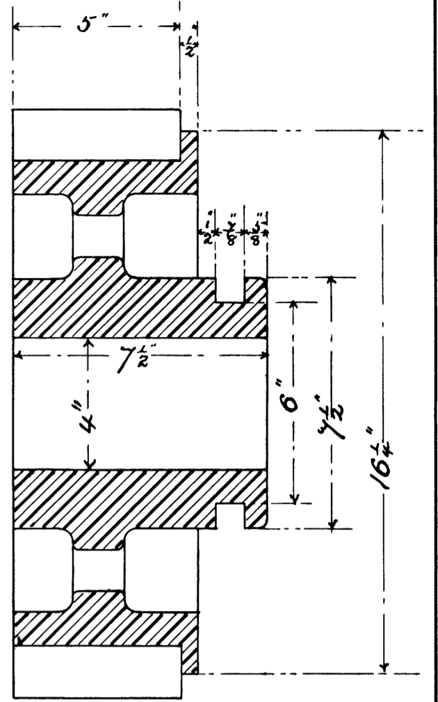
Section of 16 1/4 Pinion.
